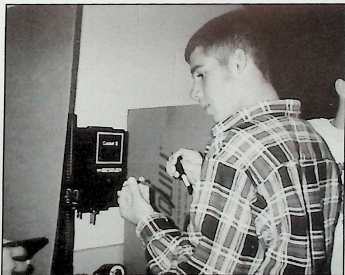
Alex Silow inserts his negatives into a special cannister. This was used for developing the negatives.
